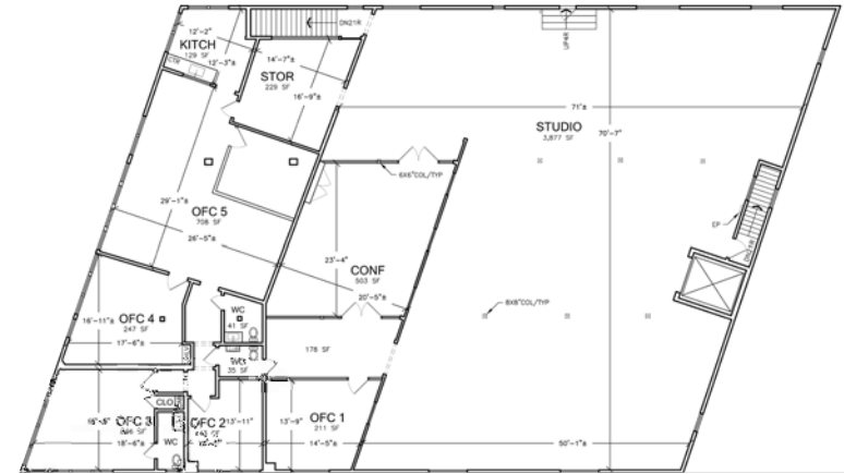
SECOND FLOOR CREATIVE OFFICE SPACE IN WAREHOUSE 2
